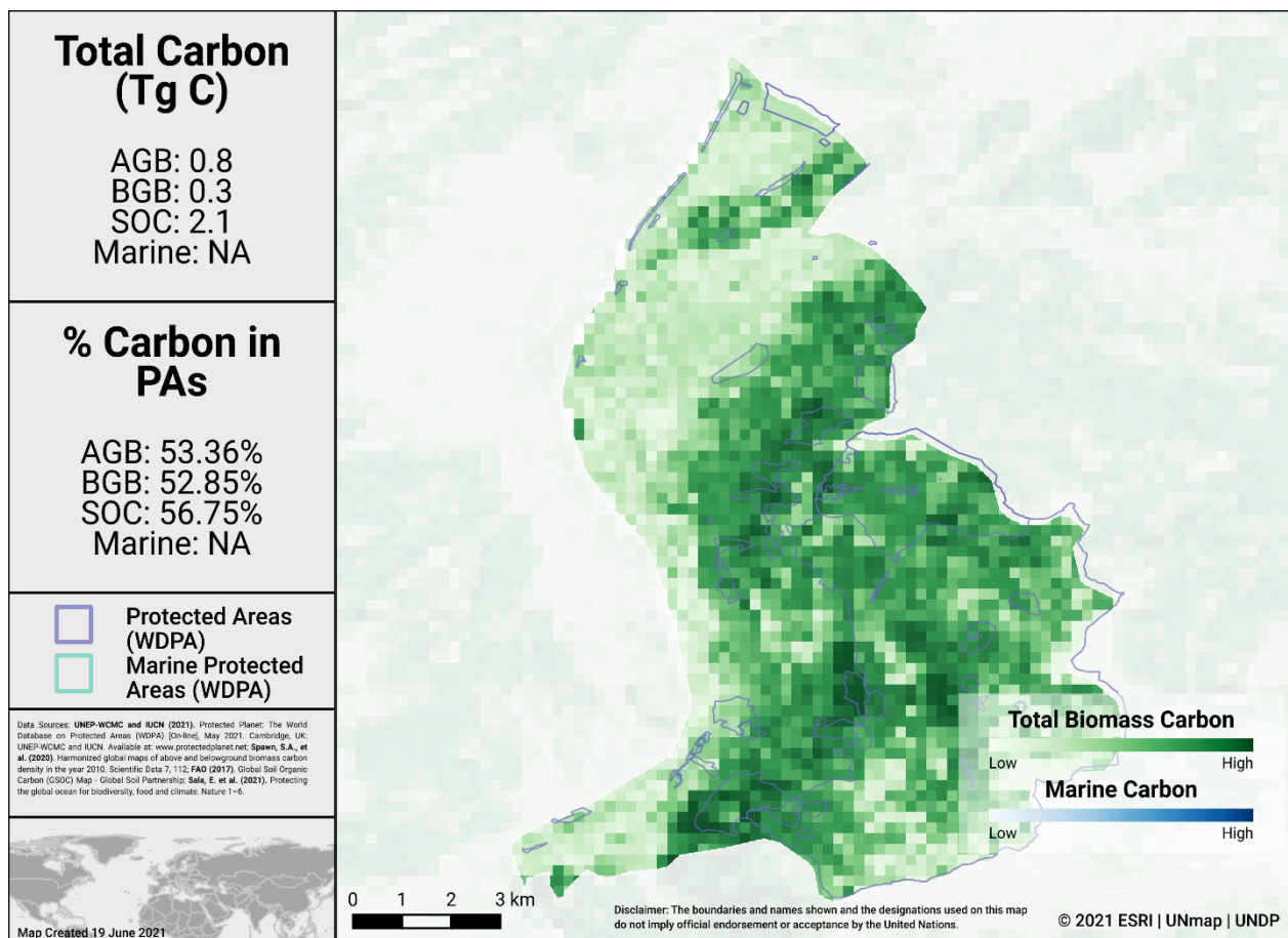
Carbon Stocks in Liechtenstein
