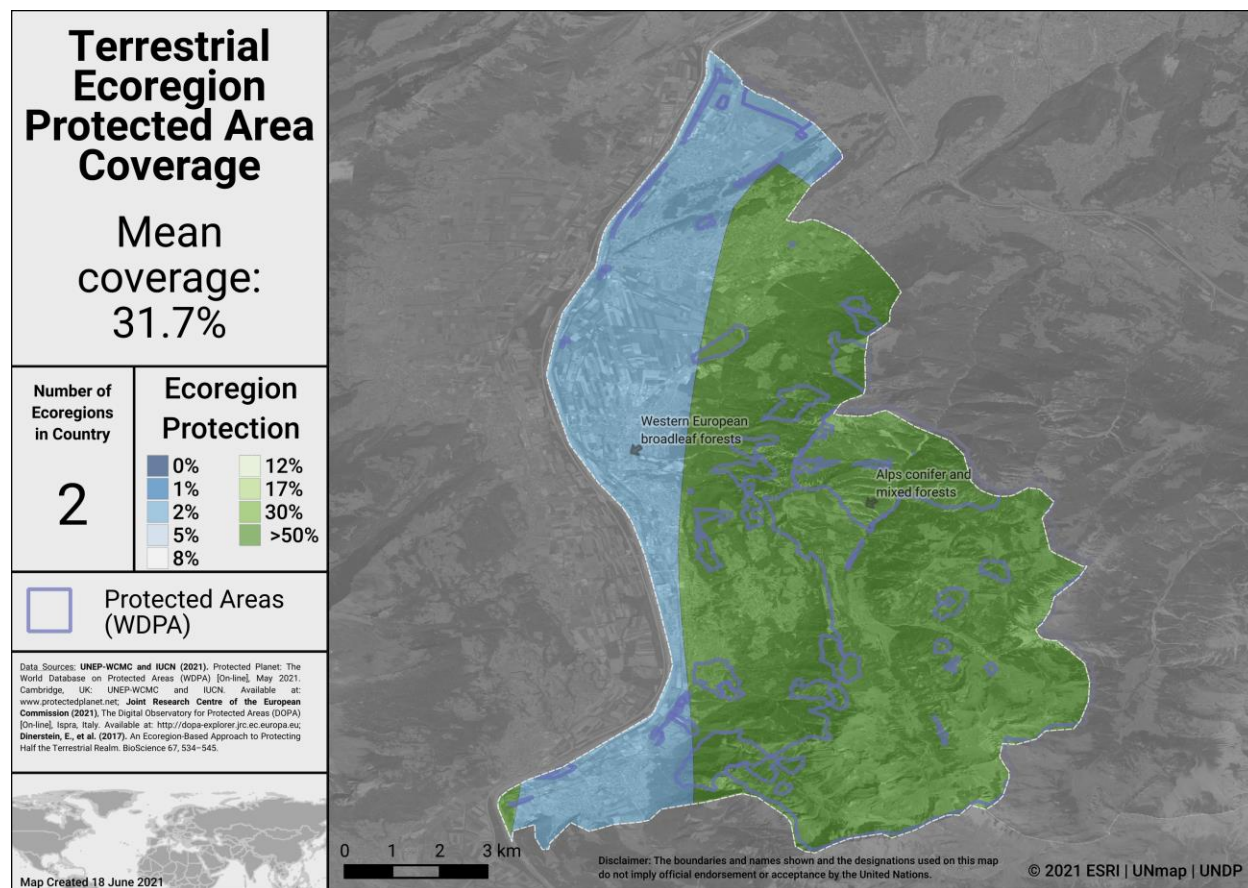
Terrestrial ecoregions in Liechtenstein
