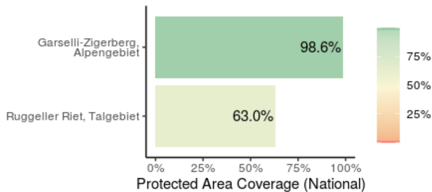
Key Biodiversity Area Coverage (KBA) in Liechtenstein
