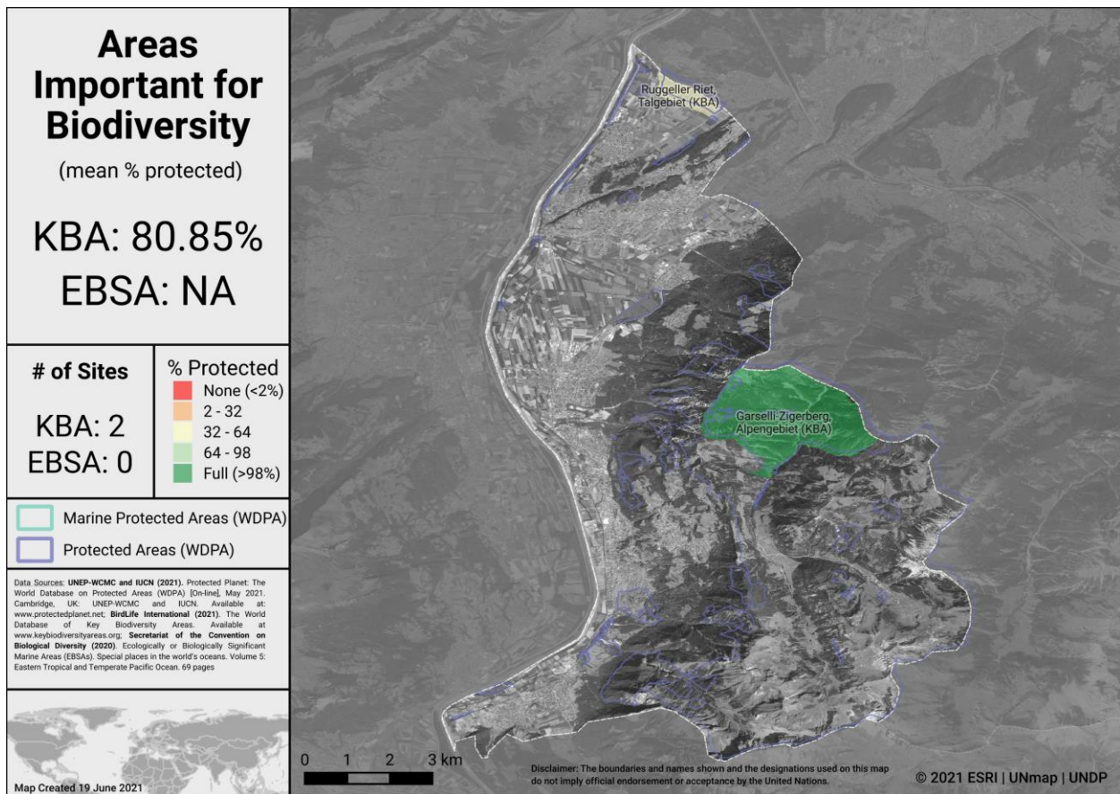
Areas Important for Biodiversity in Liechtenstein
