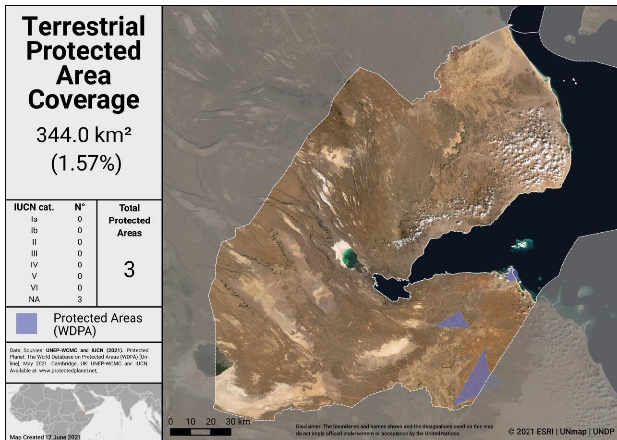
Terrestrial Protected Areas in Djibouti
