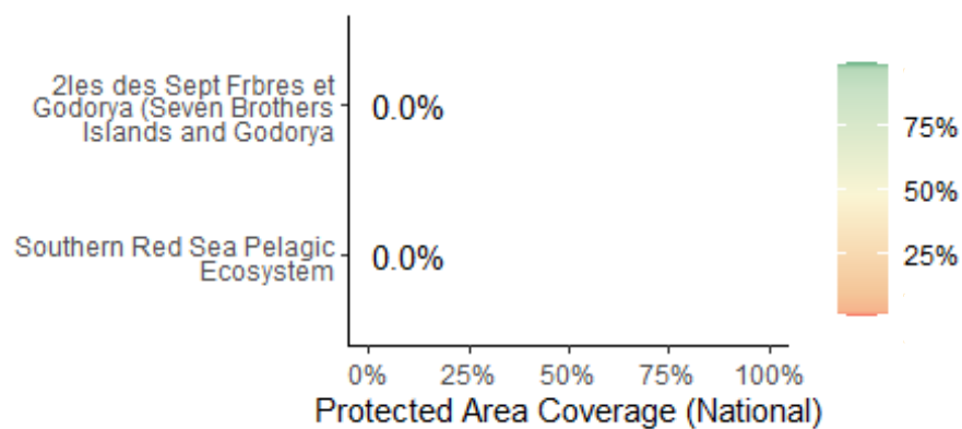
Ecologically or Biologically Significant Marine Areas (EBSAs) in Djibouti
