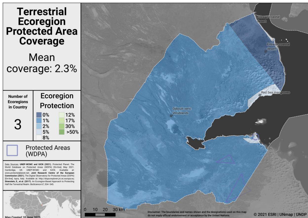
Terrestrial ecoregions in Djibouti
