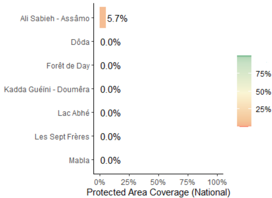
Key Biodiversity Area Coverage (KBA) in Djibouti
