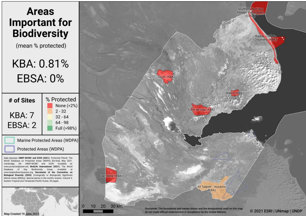
Areas Important for Biodiversity in Djibouti
