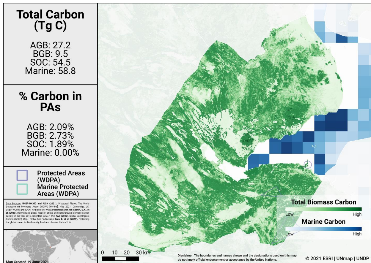
Carbon Stocks in Djibouti
