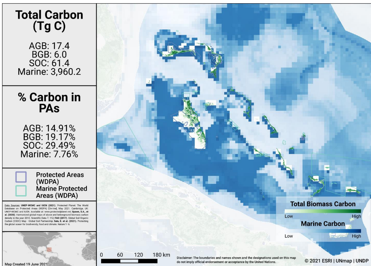
Carbon Stocks in Bahamas
