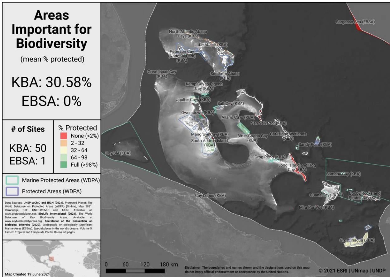
Areas Important for Biodiversity in Bahamas
