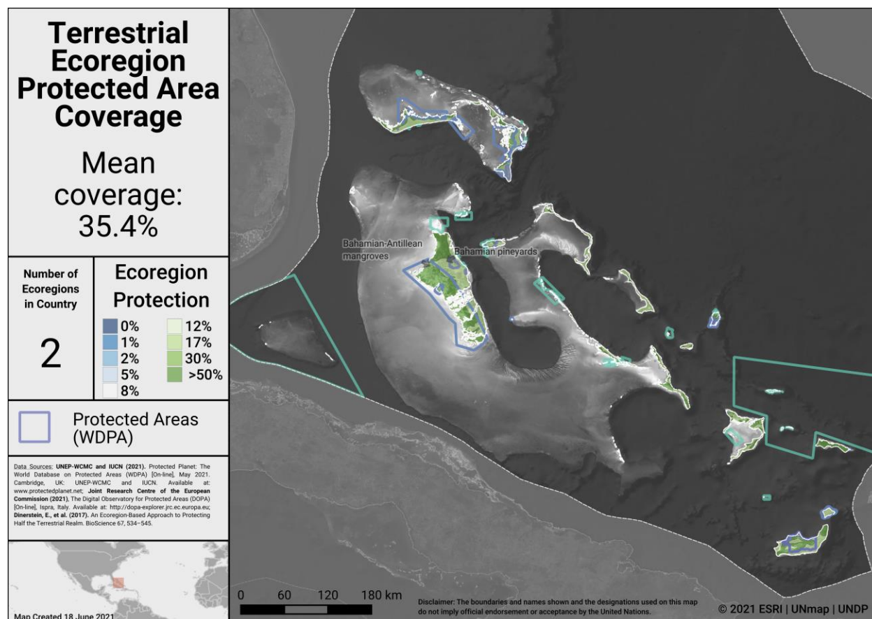
Terrestrial ecoregions in Bahamas
