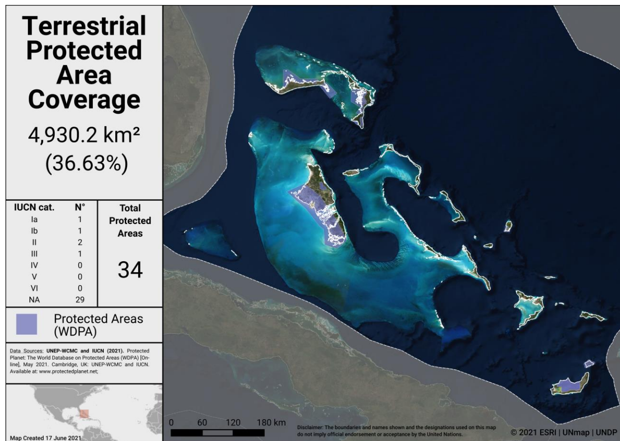
Terrestrial Protected Areas in Bahamas
