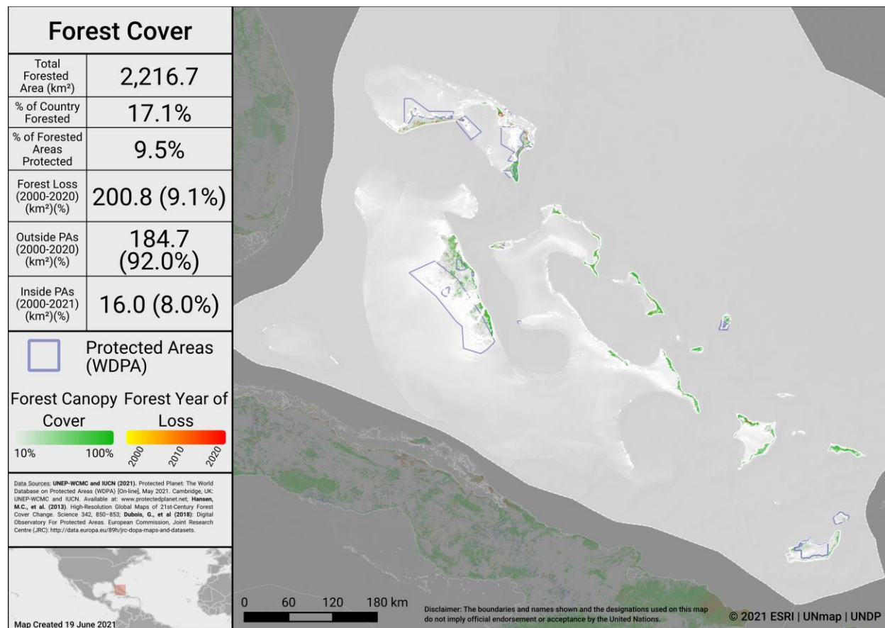
Forest Cover and Forest Loss in Bahamas
