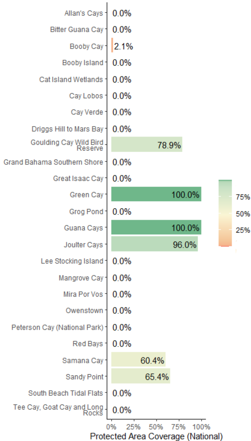
Key Biodiversity Area Coverage (KBA) in Bahamas
