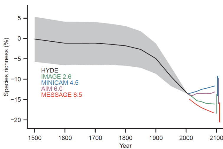
Figure 1.5 Hindcast and projected change in terrestrial local species richness 1500-2000 and 2000-2100, with the latter four pathways based on IPCC RCP 2.6, 4.5, 6.0 and 8.5. Reprinted by permission from Nature Publishing Group (MacMillan Publishers Ltd); Newbold et al. (2014) Nature 520, 45-50.
