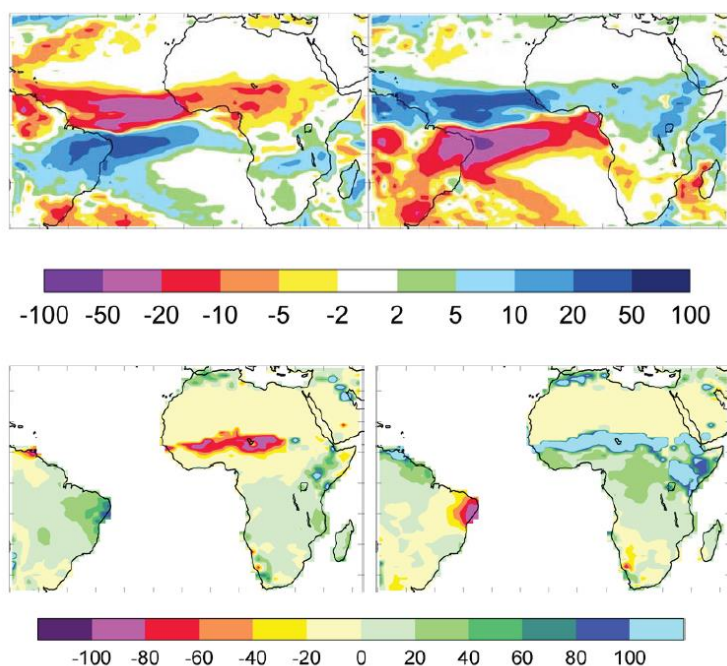
Figure 4.2 Modelled effect of hemispherically asymmetric aerosol sulphate injection. Upper maps: Change in mean precipitation (mm/month) for the period 2020-2070 when SO 2 is injected into the northern hemisphere only (left) or southern hemisphere only (right) in comparison to RCP 4.5 scenario. Lower maps: Percentage change in net primary production under the same conditions. Reprinted by permission from Nature Publishing Group (MacMillan Publishers Ltd); Haywood et al. (2013) Nature Climate Change 3, 660-665.
