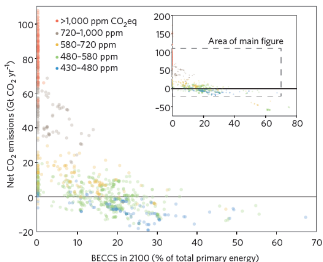
Figure 3.1. The importance of BECCS in limiting net CO 2 emissions and atmospheric CO 2 eq concentrations in climate change scenarios. Data from IPCC AR5 database, Global Carbon Project and Carbon Dioxide Information Analysis Centre. Reprinted by permission from Nature Publishing Group (MacMillan Publishers Ltd); Fuss et al (2014) Nature Climate Change 4, 850-853...
